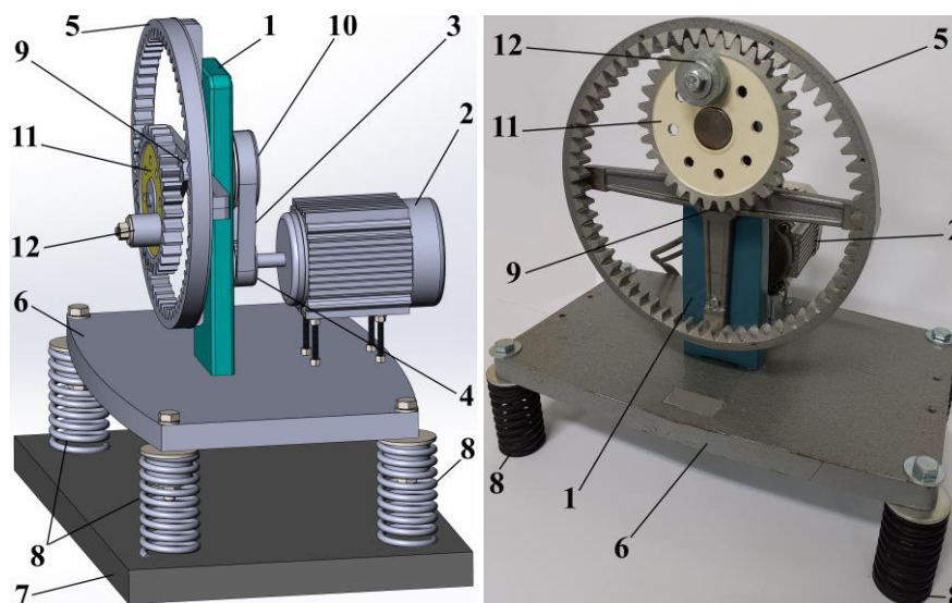
Fig. 7. Single-stage planetary-type vibratory exciter: structural components and assembly [12]: 1 - planetary-type mechanism, 2 - electric motor, 3 - toothed belt transmission, 4 - driving pulley, 5 - ring gear, 6 - machine's body, 7 - stationary support surface, 8 - set of four coil-type cylindrical springs, 9 - planet carrier, 10 - driven pulley shaft, 11 - planet gear, 12 - unbalanced mass [12]
