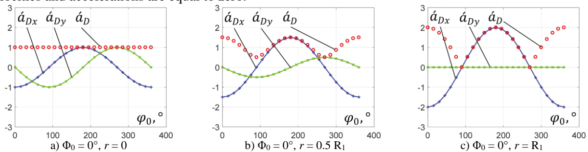
Fig. 10. Acceleration components of the unbalanced mass [12]
