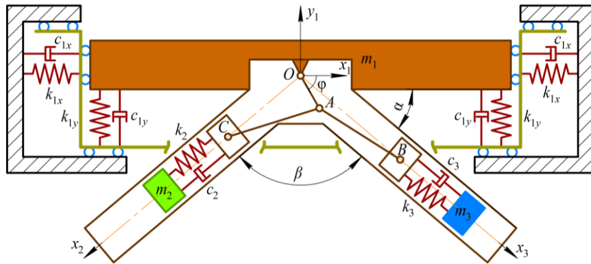
Fig. 17. Dynamic model of the vibratory system [16]
