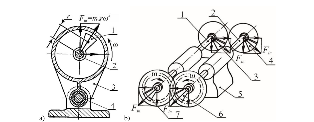
Fig. 2. a) Pendulum vibratory exciter b) Four-mass vibratory exciter [1]
