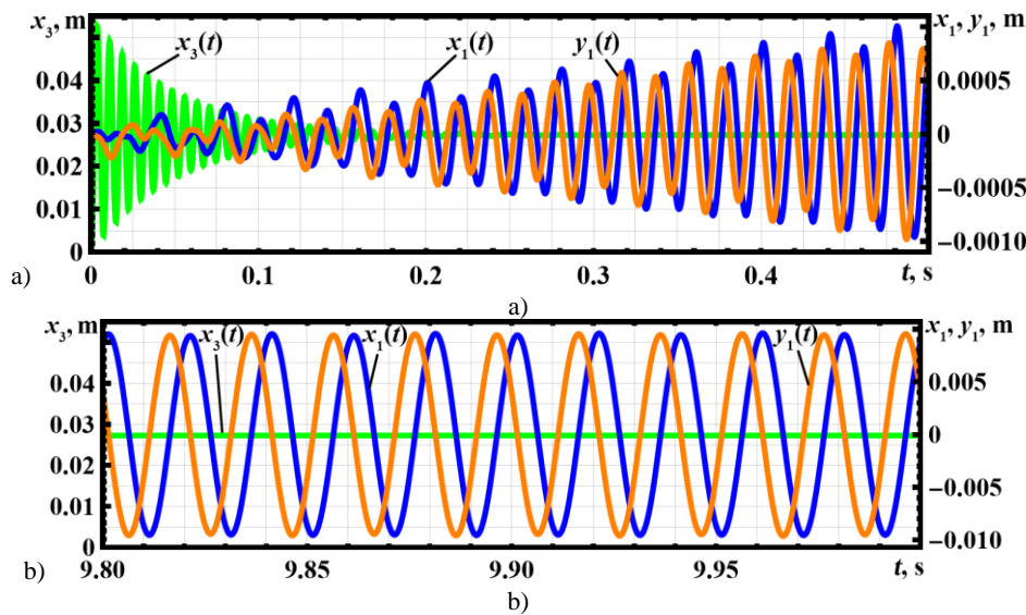
Fig. 13. Oscillatory motion of masses over time: a) initial phase t = 0 \dots 0.5 s; b) steady-state phase t = 9.8 \dots 10 s [13]
