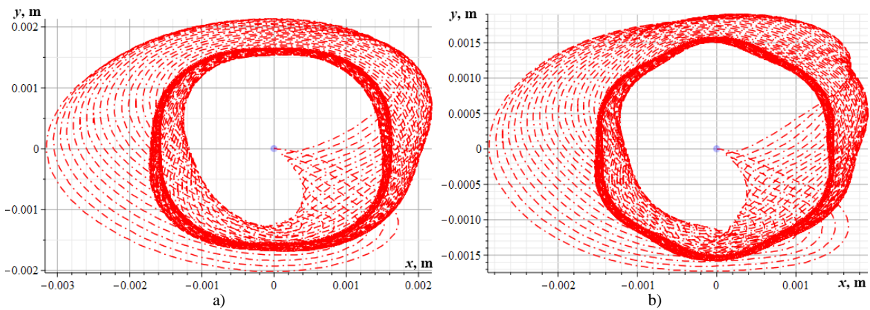
Fig. 6. Trajectories of the unbalanced mass motion for different geometric parameters of the planetary-type vibration exciter [11]
