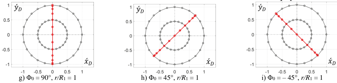
Fig. 8. Influence of initial conditions and geometric ratios on motion trajectories of the unbalanced mass [12]
