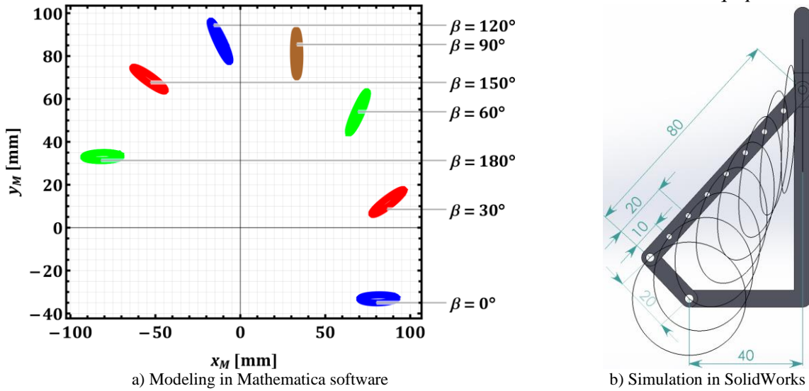
Fig. 16. Motion trajectories of the connecting rod point under different angles \beta and link dimensions l_2 and l_3 [15]
