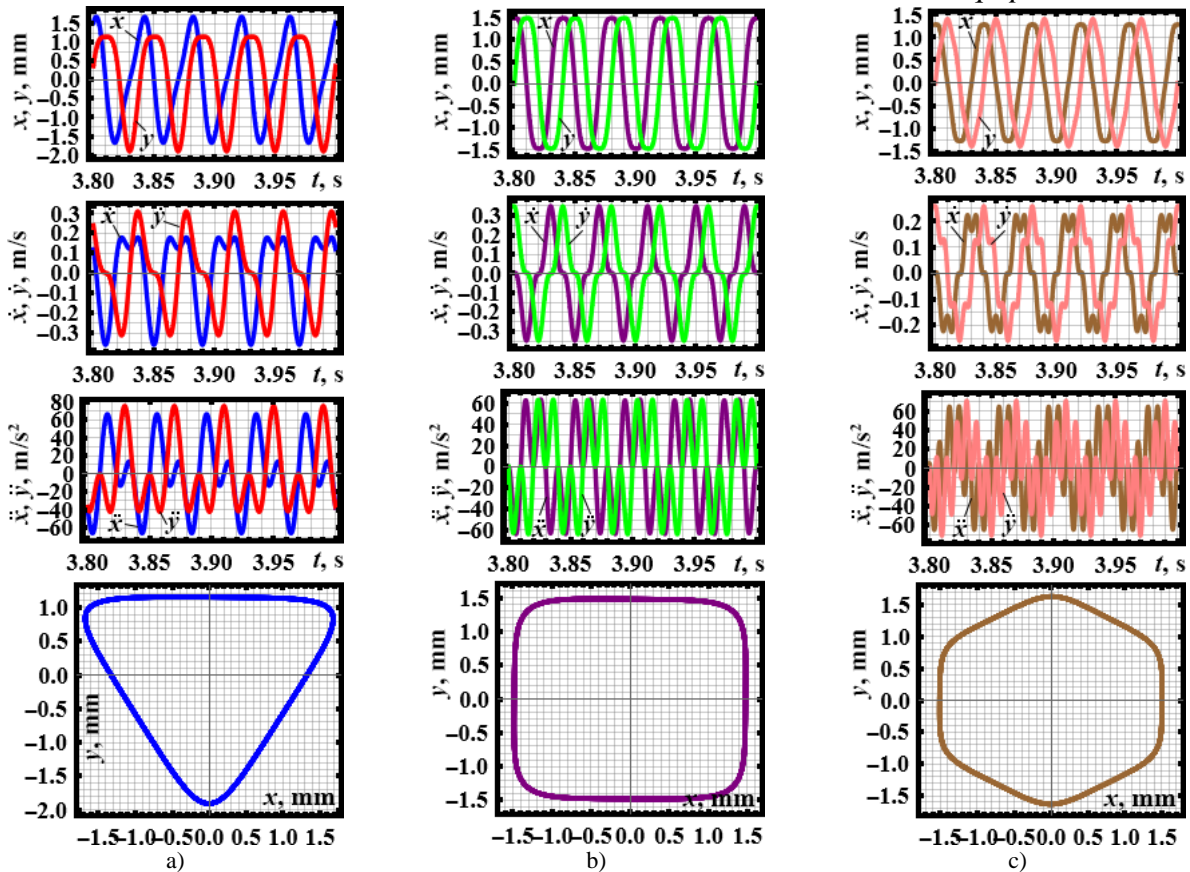
Fig. 5. Motion analysis of the system with varying planetary-type exciter design parameters [11]
