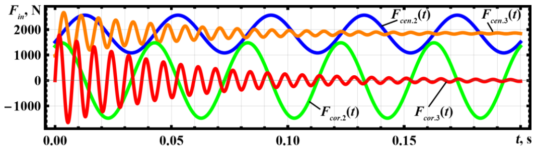
Fig. 12. Force-time dependencies of vibration exciter's oscillating bodies [13]
