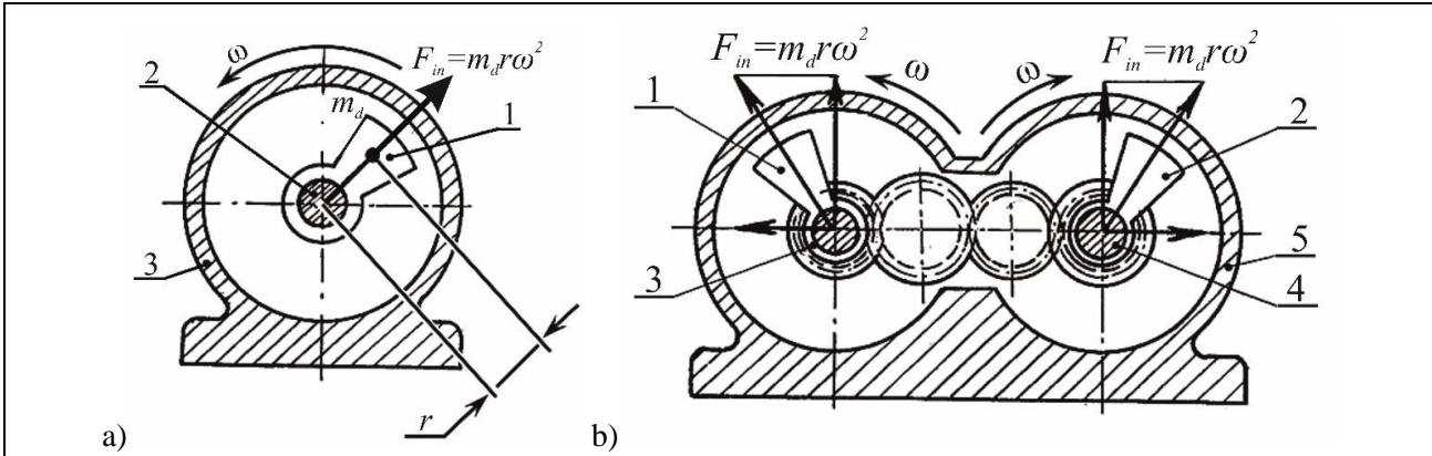
Fig. 1. a) Unbalanced vibration exciter b) Self-balancing vibration exciter [1]
