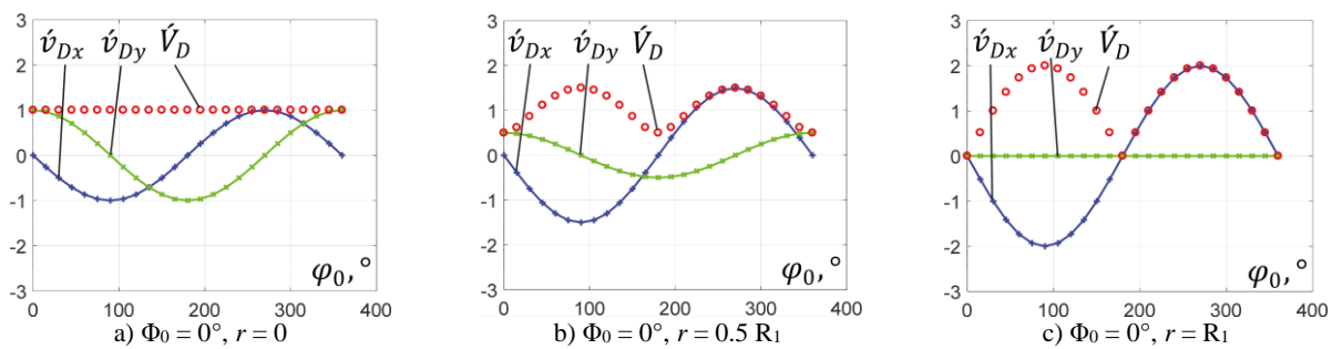
Fig. 9. Speed characteristics of the unbalanced mass [12]
