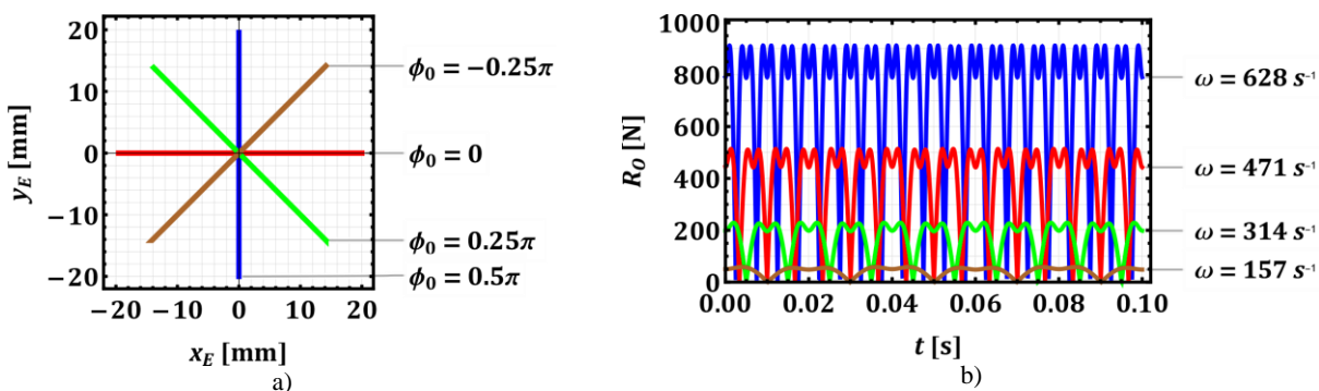
Fig. 14. Dependence of the imbalanced body trajectory a) and central hinge reactions b) on carrier inclination angles and carrier angular speeds
