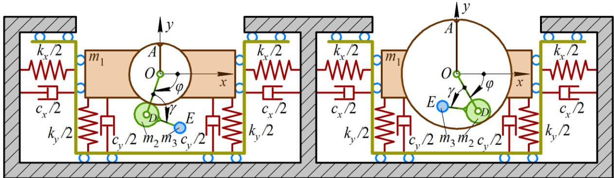
Fig. 4. Schematic representation of a single-mass vibratory system with planetary-type exciters [11]
