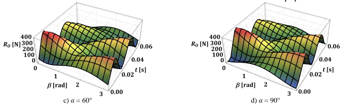
Fig. 21. Reaction force - time dependencies at different \alpha and \beta angles in the central hinge [17]
