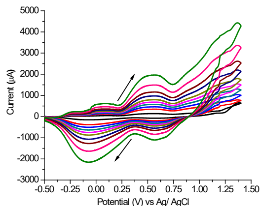
Fig. 1 Cyclic voltammogram resulting from electropolymerisation of 10 mM EDOT/Schiff base with 0.1 M Bu 4 NPF 6 in DCM solution between -0.5 and 1.4 V at 10 mV s -1 for 10 scans. Electrode area was 0.00785 cm 2 .
