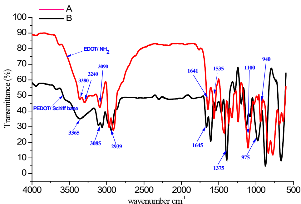
Fig. 5 FTIR spectra of A) synthesised monomer (red line) and B) synthesised poly(EDOT/Schiff base) (black line).
