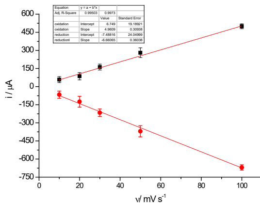
Fig. 4 Variation of redox peak current A) from Figs. 3B and B) from Fig. 3D with scan rate (in the range 10-100 \text{mV s}^{-1} ).
