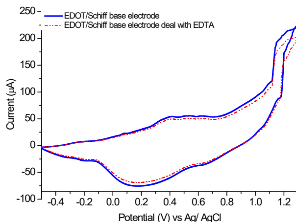
Fig. 13 Cyclic voltammetric of PEDOT/Schiff modified electrode (blue curve) in \text{Bu}_4\text{NPF}_6 aqueous electrolyte (red curve) after treating with 0.1 M EDTA
