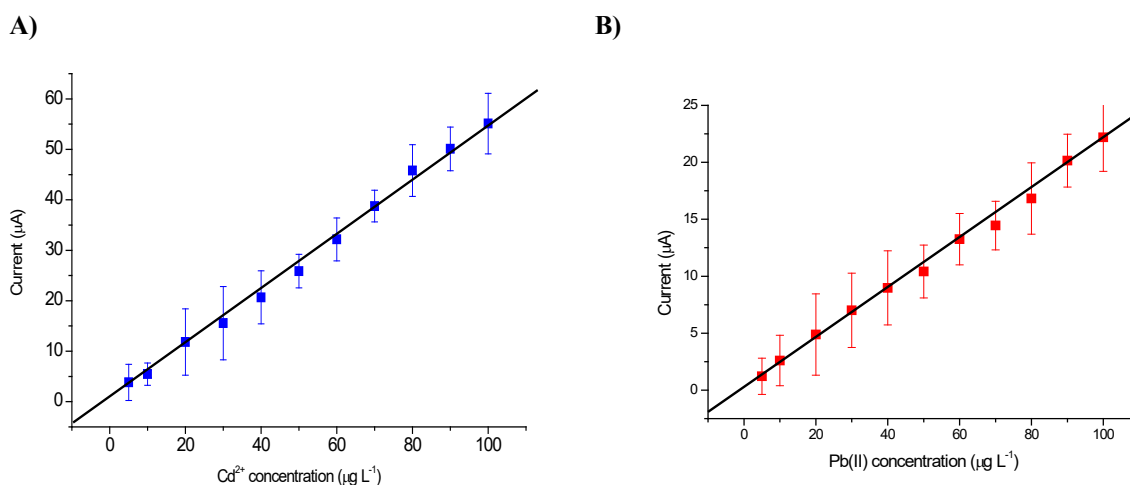
Fig. 10 Calibration plot for measurement of different concentrations (5 - 100 \mu\text{g L}^{-1} ) of (A) Cd(II) and (B) Pb(II) taken from Fig. 9 using a poly(EDOT/ Schiff) electrode.
