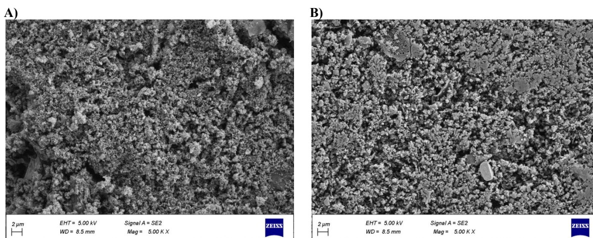
Fig. 6 SEM images of (A) poly(EDOT/Schiff) formed using electropolymerisation at a scan rate 10 \text{ mV s}^{-1} before adsorption, and (B) poly(EDOT/Schiff) after adsorption of metal ions (see the conditions in Fig. 11).
