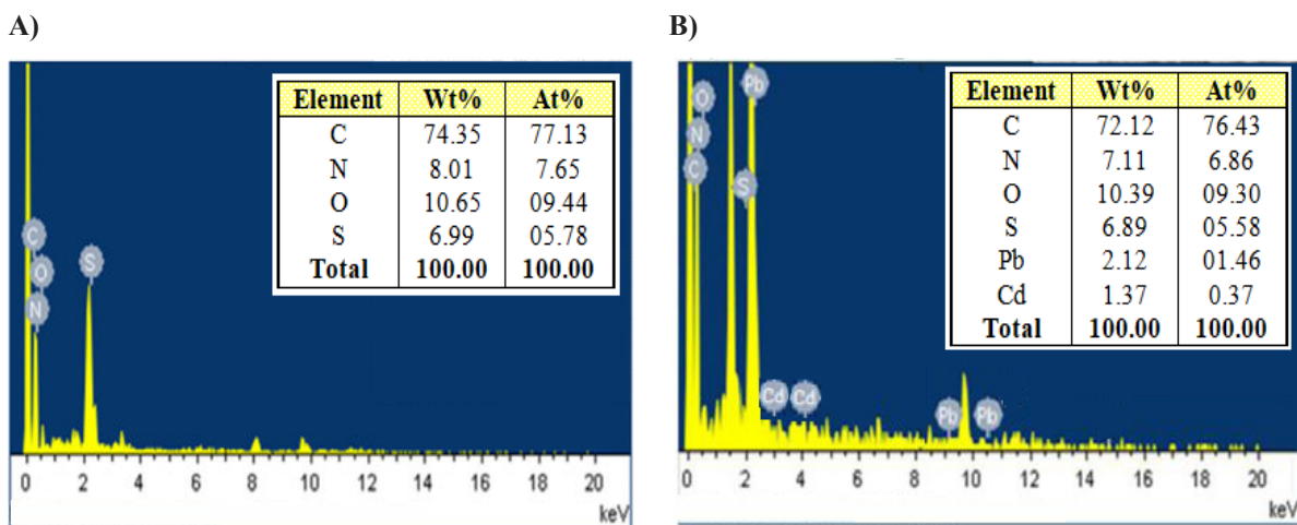
Fig 12 EDX spectra showing elemental analysis of poly(EDTA/Schiff base) (A) before and (B) after adsorption of metal ions.
