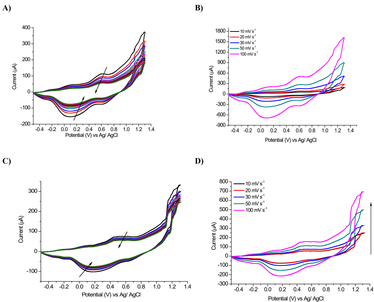
Fig. 3 Voltammetric response of poly(EDOT/Schiff) electrodes prepared at 10 \text{mV s}^{-1} ( Figure 1 ) and acquired in A ) 0.1 M \text{Bu}_4\text{NPF}_6 in DCM, and C ) 0.1 M \text{Bu}_4\text{NPF}_6 in the aqueous electrolyte (monomer-free) at -0.5 to 1.3 V. Voltammetric responses of the same polymer film at various scan rates in the range 10-100 \text{mV s}^{-1} B ) DCM and D ) aqueous electrolyte.
