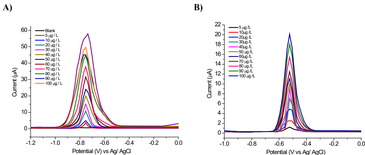
Fig. 9 SWV curves for different concentrations of (A) Cd(II) and (B) Pb(II) from lower to higher concentration ( 5 - 100 \mu\text{g L}^{-1} ) using a poly(EDOT/Schiff) electrode.
