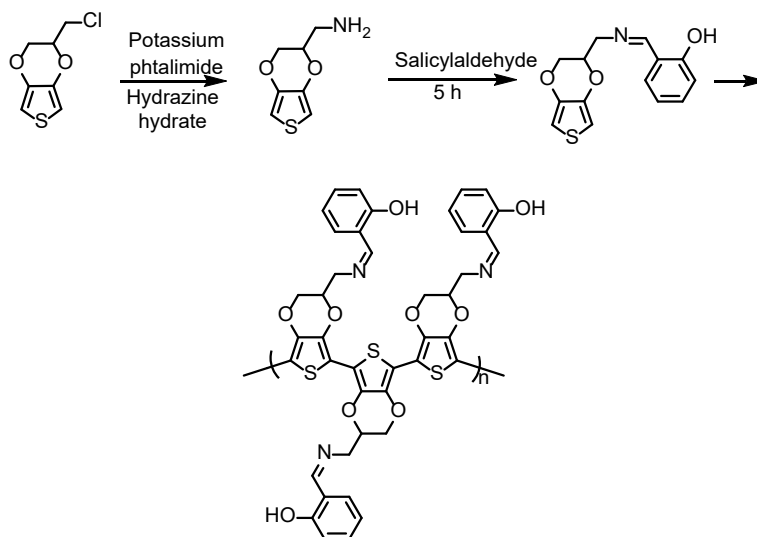
Scheme 1 The synthesis of the monomer EDOT/ Schiff base and the polymerisation reaction
