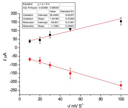
Fig. 4 Variation of redox peak current A) from Figs. 3B and B) from Fig. 3D with scan rate (in the range 10-100 \text{mV s}^{-1} ).
