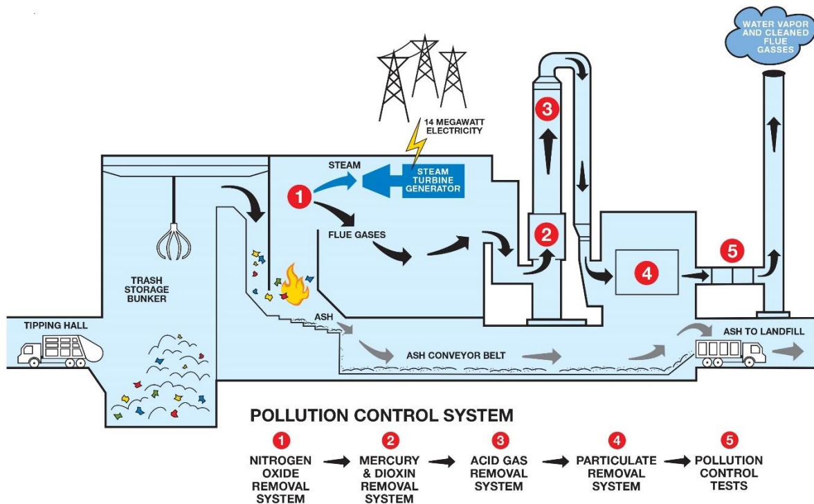
Figure 2: A Typical Waste to Energy Plant
