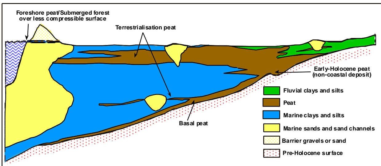
Fig. 2. Schematic representation of the stratigraphic architecture of the coastal peat deposits of the southern North Sea region.
