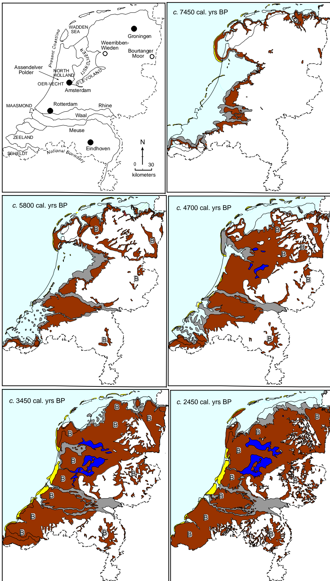
Fig. 7. Location of sites and palaeographic maps from the Netherlands (after Vos, 2015). See Fig. 9 for key.
