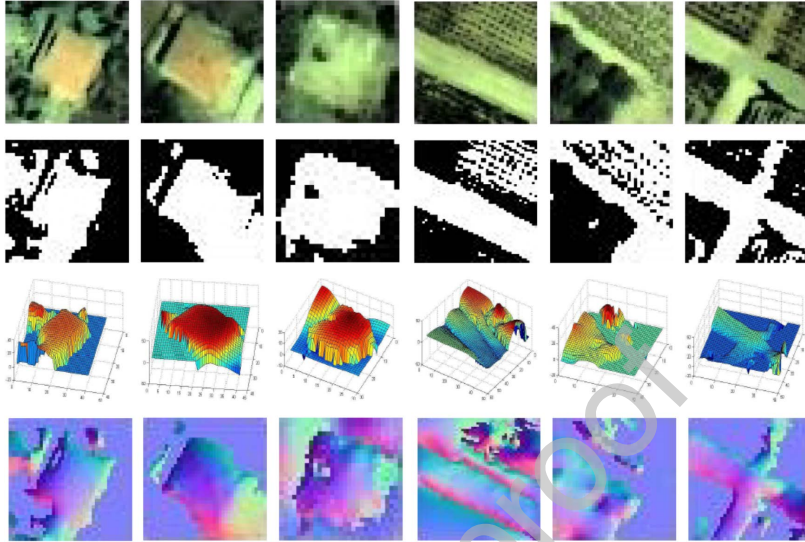
Figure 5: Examples of the 3D reconstructed buildings and the corresponding height and normal maps.
