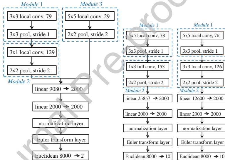
Figure 3: Optimal Modular-CNN architectures for the (a) QuickBird/WorldView-2, (b) CIFAR-10 and (c) MNIST datasets.
