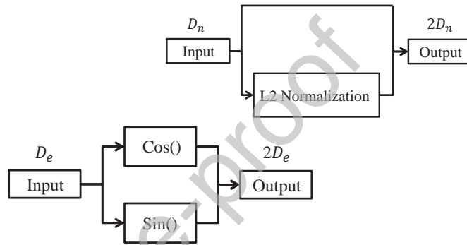
Figure 2: Proposed Normalisation (top) and Euler transform (bottom) layers.
