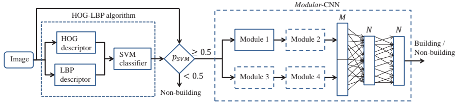
Figure 1: Flowchart of the proposed building detection methodology.
