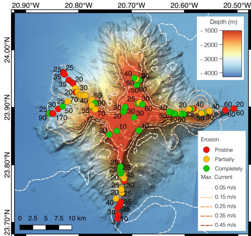
Figure 7: Sample locations coloured according to erosion state defined from SEM images of surface textures. Contours are the maximum current magnitude extracted from the hydrographic model. All data is overlaid on the EM120 bathymetry gridded at 100 m. Black numbers are measured FeMn crustal thicknesses in mm.
