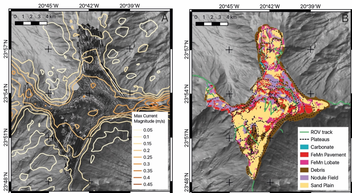
Figure 4: (A) Sidescan sonar data of the summit collected by AutoSub6000, mosaicked at 2 m, overlaid on the EM120 bathymetry of Tropic seamount gridded at 100 m. Maximum current magnitudes are shown by the contours. (B) Geological map of the surface outcrop at Tropic Seamount. Grey dashed lines show the locations of summit plateaus, probably formed by
