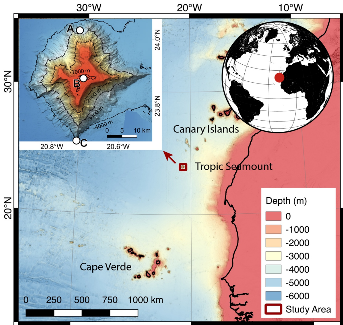
Figure 1: Location of Tropic Seamount, which is a guyot rising from a 4000 m deep abyssal seafloor to a summit depth of 1100 – 900 m. Regional bathymetry is extracted from Sandwell et al. (2014) gridded at 30 seconds. Inset shows EM120 bathymetry collected during expedition JC142, and gridded at 100 m. Gaps have been filled using the Sandwell et al. (2014) grid. White dots A – C are mooring locations for current measurements.
