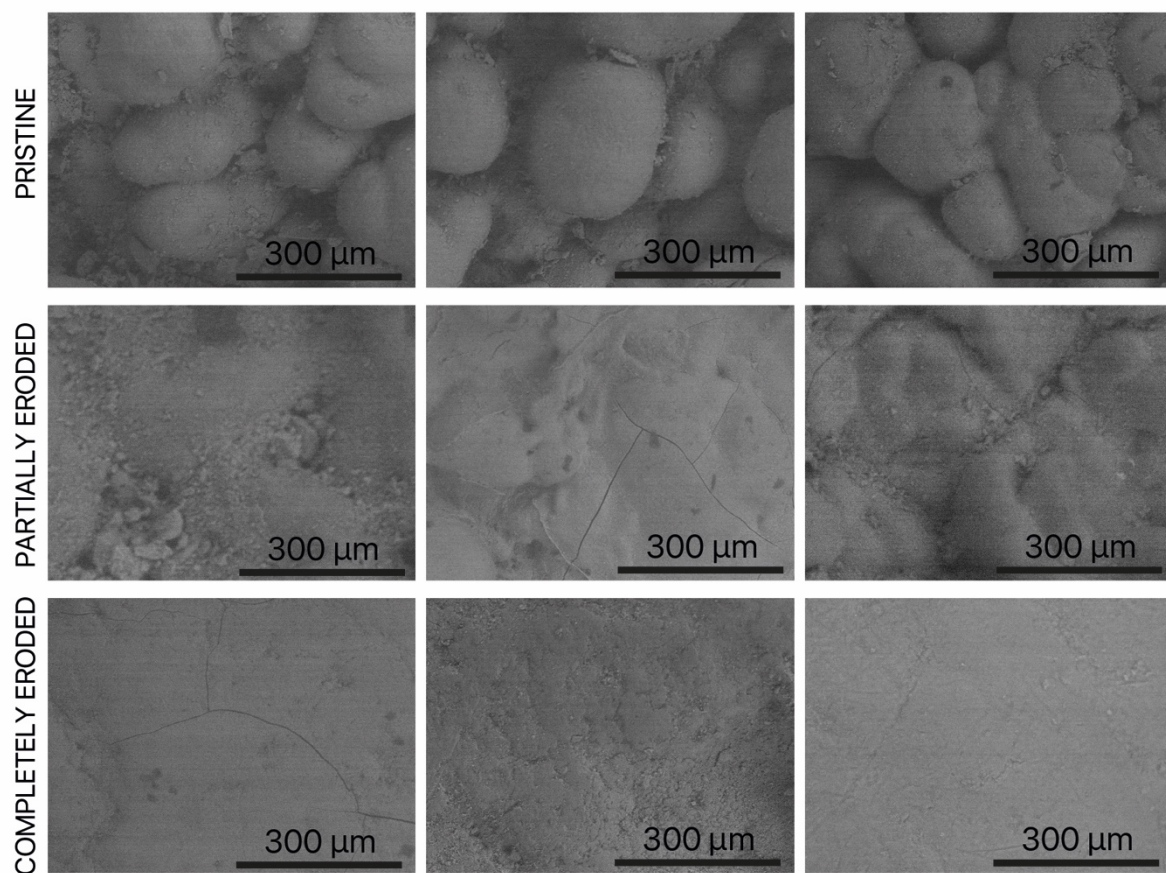
Figure 2) SEM images showing representative surface textures and the way they are categorised. All samples with detailed botryoidal growth surfaces are classified as pristine, those totally planed flat as completely eroded and those somewhere in between as partially eroded. Images are all shown at the same scale.
