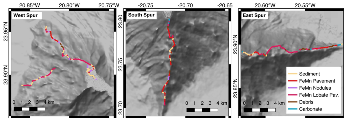
Figure 6: Surface lithology logged from ROV video up three spurs of Tropic Seamount. No observations were made on the northern spur. Observations are overlaid on the EM120 bathymetry gridded at 100 m. All maps are shown at the same scale.
