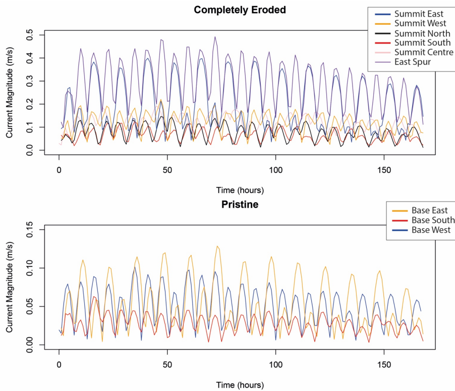
Figure 3: Representative current magnitude profiles extracted for a week-long period at sampling locations around the seamount. The upper graph shows profiles only for samples classed as heavily eroded, and the lower graph for samples in pristine condition.
