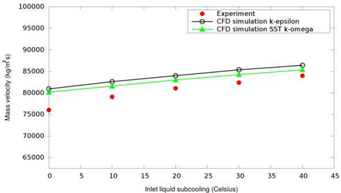
Fig. 4: Predicted mass flow rates per unit area for initial pressure equal to 160 bar compared to experimental data of Xu et al. (1995).
