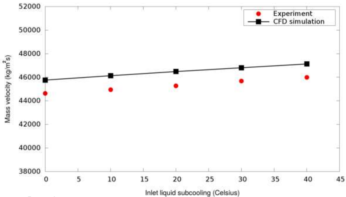
Fig. 2: Predicted mass flow rates per area for initial pressure equal to 40 bar compared to experimental data of Xu et al. (1995).
