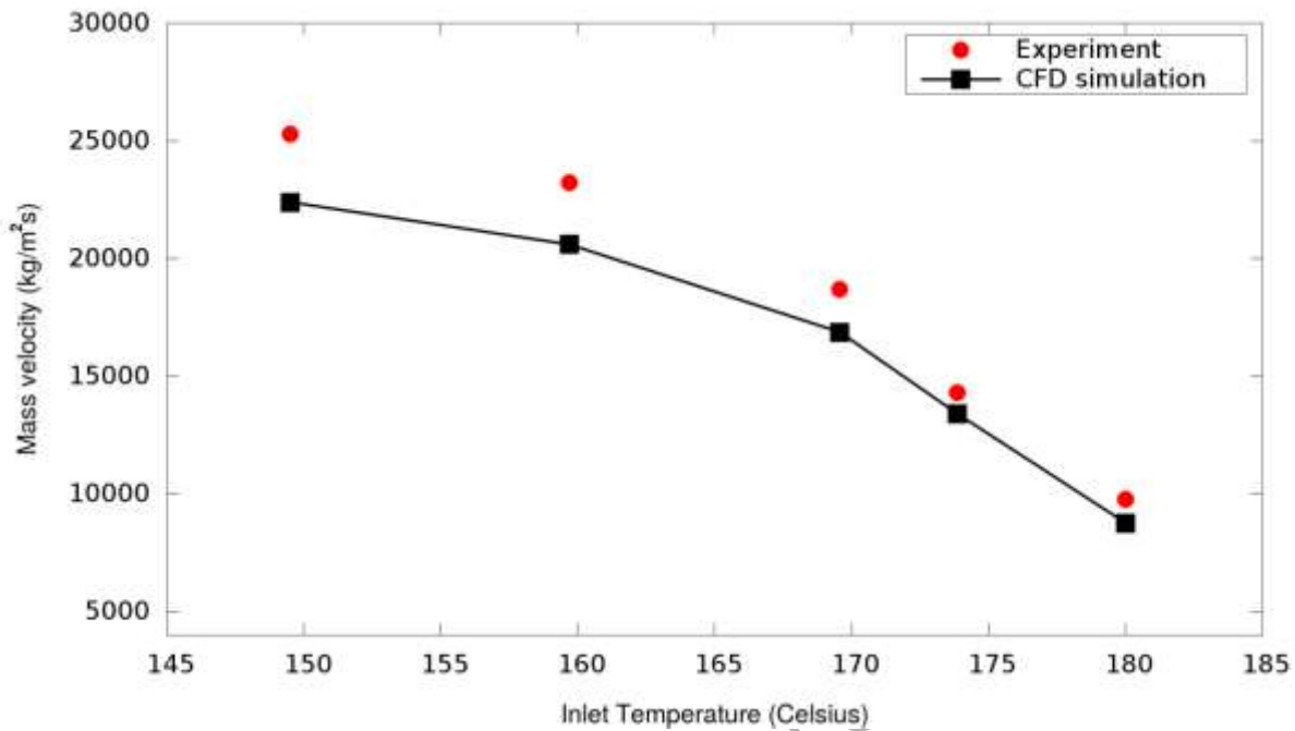
Fig. 8: Predicted mass flow rates per area for different initial temperatures compared to experimental data of Park et al. (1997).
