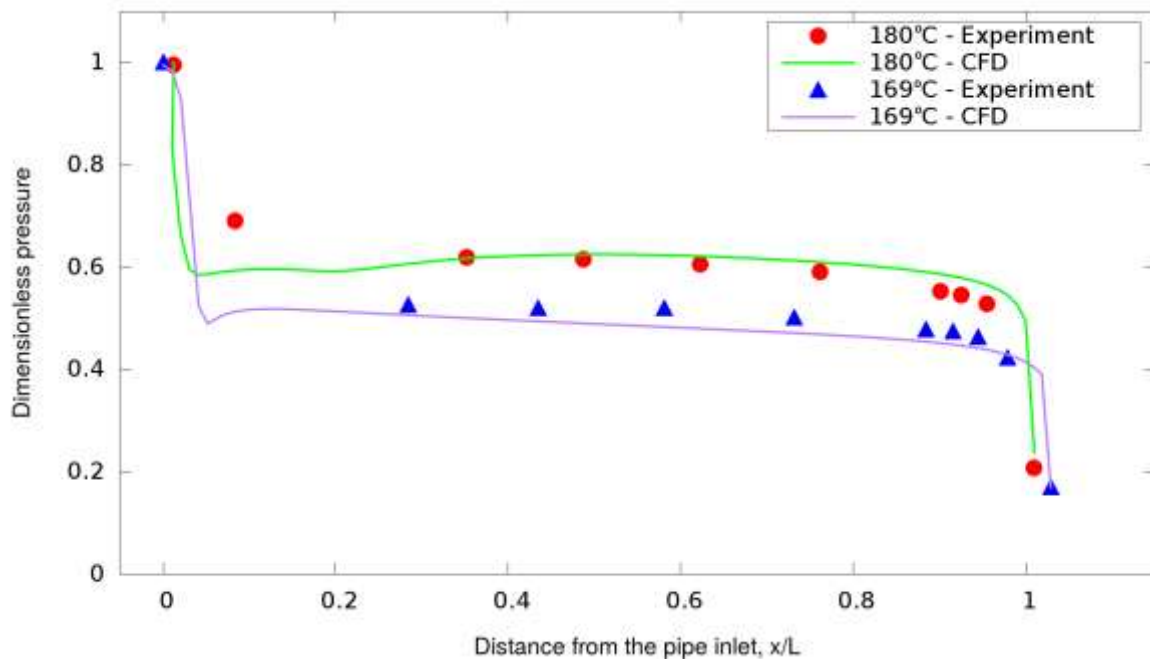
Fig. 9: Predicted pressure distribution along the pipe for different inlet temperatures for L/D=29.4.
