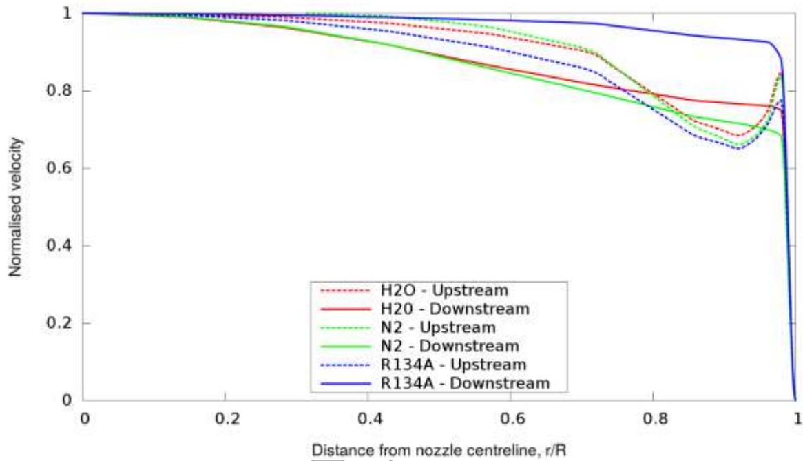
Fig. 12: Normalised velocity for liquid Nitrogen, R134A and water at atmospheric releases for inlet pressure 8 bar and L/D = 2 .
