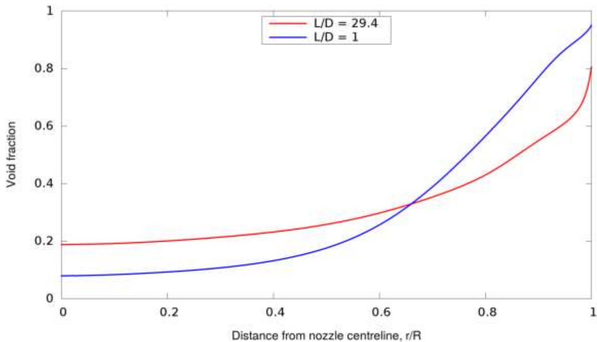
Fig. 11: Predicted void fraction for inlet pressure equal to 15 bar and different L/D for water flow.
