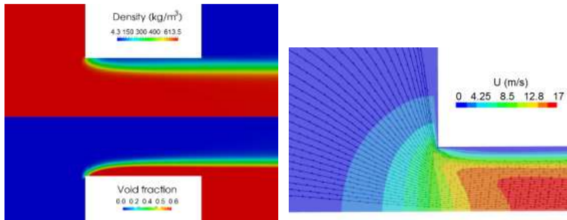
Fig. 3: Predicted instantaneous contours of the mixture density, void fraction and velocity profile for the case of 40 bar at the saturated conditions with same configuration as in the experiment of Xu et al. (1995).
