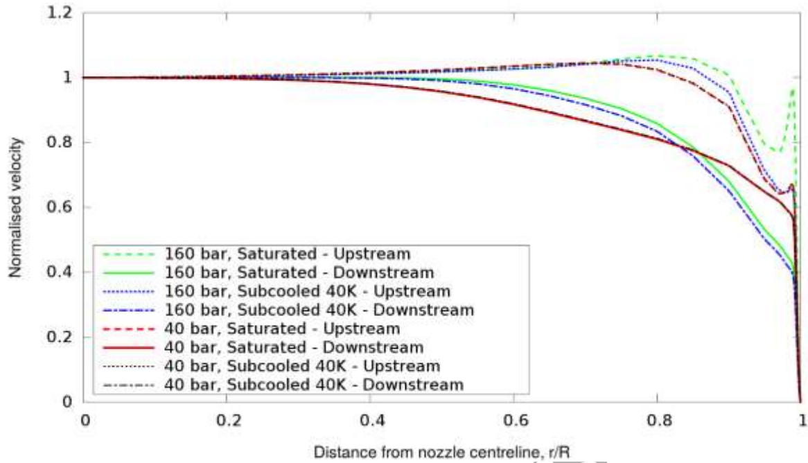
Fig. 5: Predicted velocities for different inlet pressures and temperatures upstream-downstream the nozzle.
