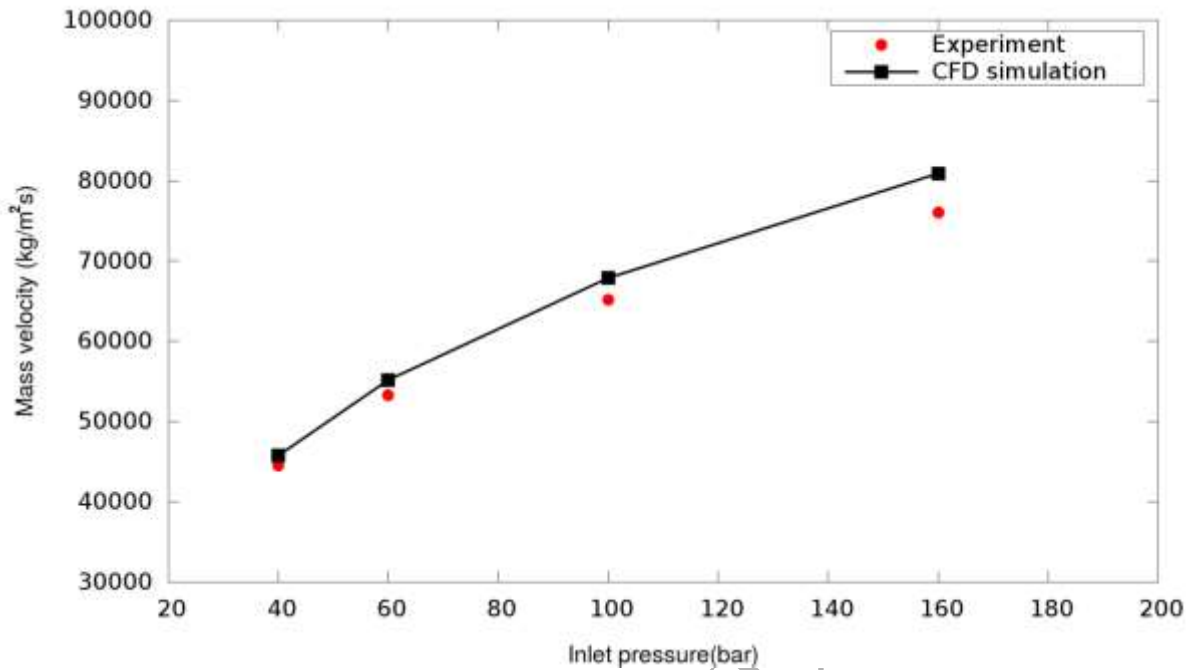
Fig. 6: Predicted mass flow rates per area for saturated stagnation conditions and different initial pressures up to 160 bar compared to experimental data of Xu et al. (1995).
