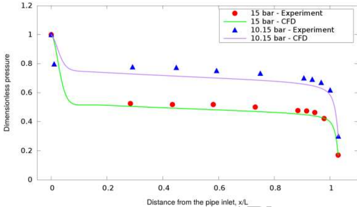
Fig. 10: Predicted pressure distribution inside the pipe for 169.4 °C and different initial pressures.
