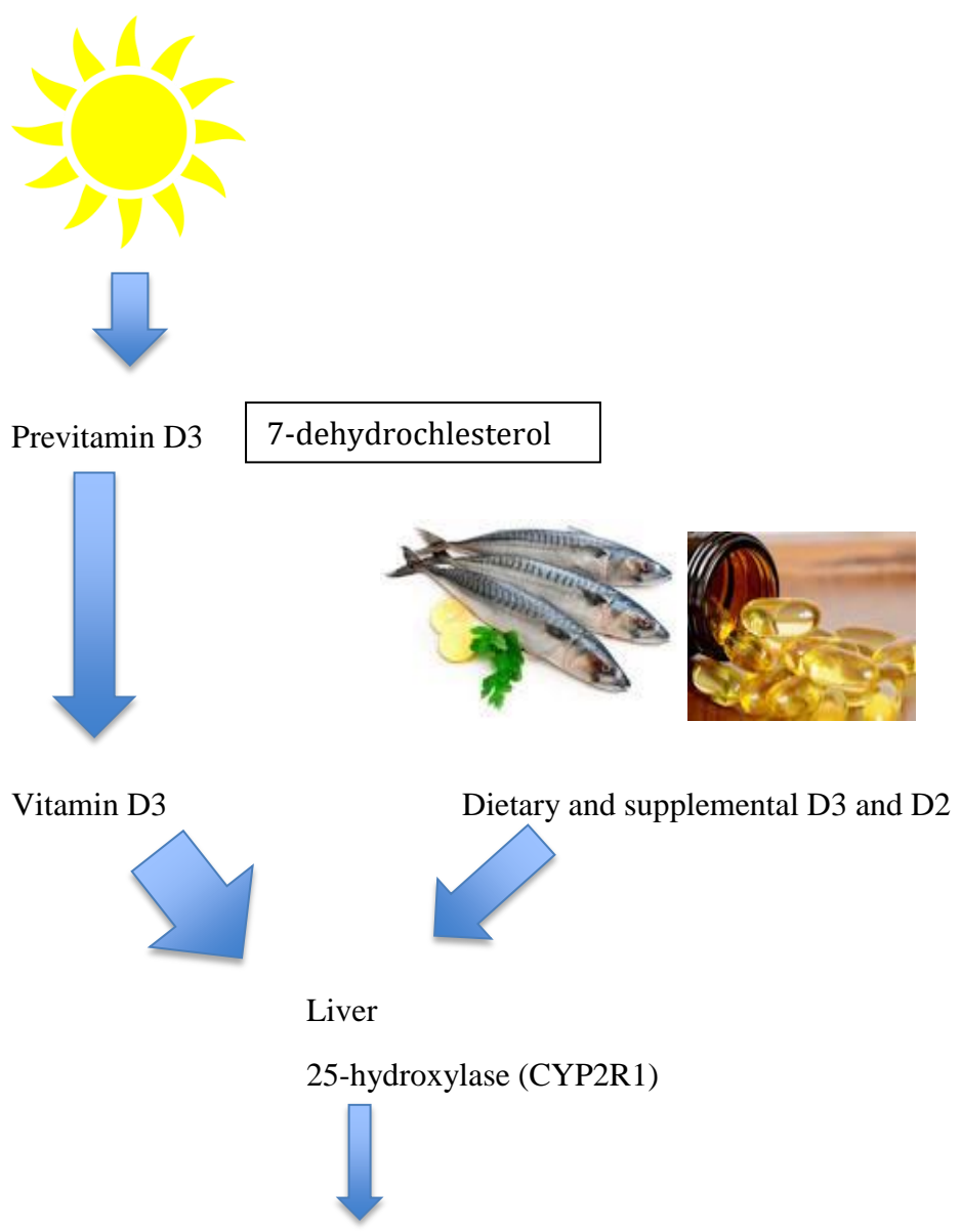
Figure 1: Vitamin D metabolism pathway (Modified from SACN (2015)).
