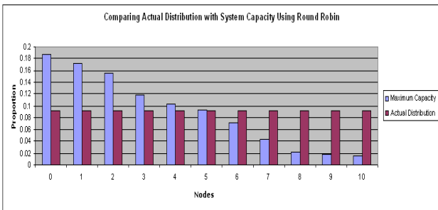
Fig. 19. Round Robin Distribution vs. System Capacity
