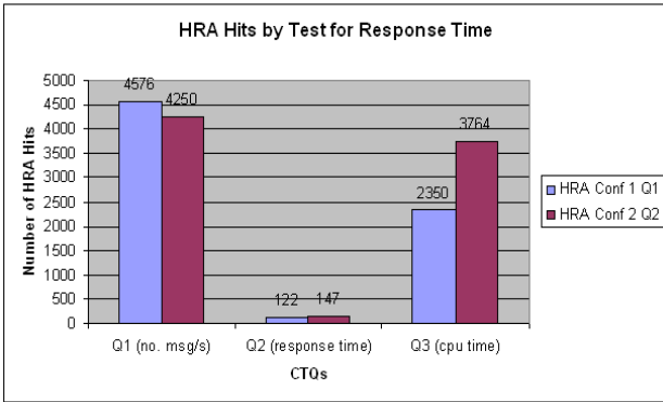
Fig. 12. Response Time Adaptability to AHP Trend
