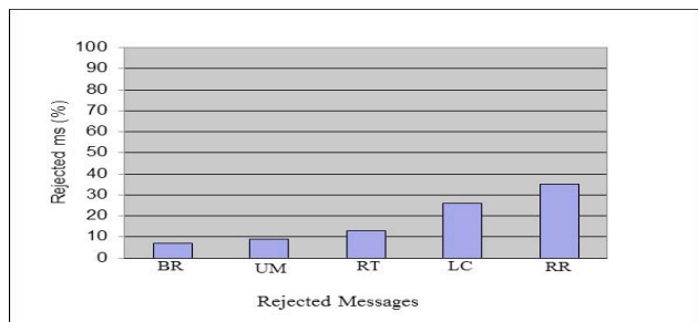
Fig. 22. Rejected messages rate of the five algorithms
