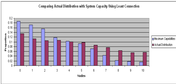
Fig. 18. Least Connections Distribution vs. System Capacity
