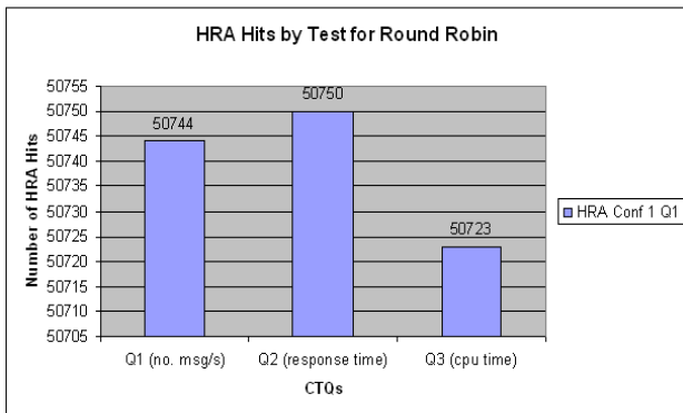
Fig. 14. Round Robin Adaptability to AHP Trend
