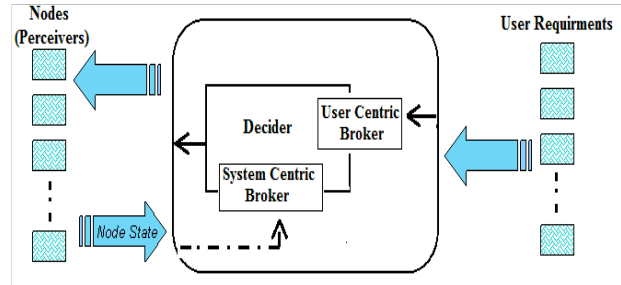
Fig. 3. Illustrative model of the Decider
