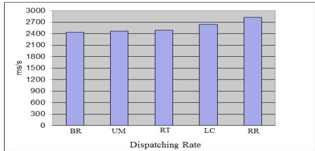
Fig. 21. Dispatching rate of the five algorithms
