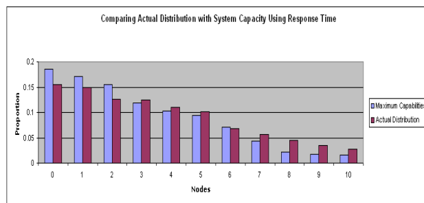
Fig. 17. Response Time Distribution vs. System Capacity
