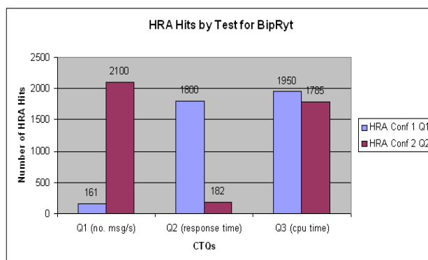
Fig. 11. BipRyt Adaptability to AHP Trend
