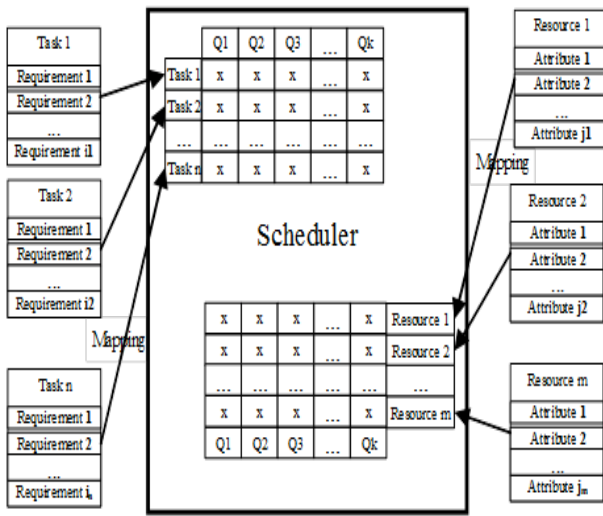
Fig. 7. A Matching Mechanism
