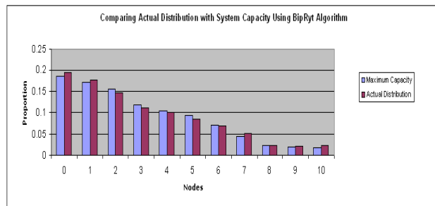
Fig. 16. BipRyt Distribution vs. System Capacity
