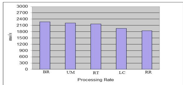
Fig. 23. Processing rate of the five algorithms
