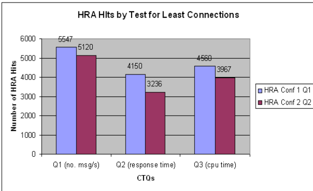
Fig. 13. Least Connections Adaptability to AHP Trend
