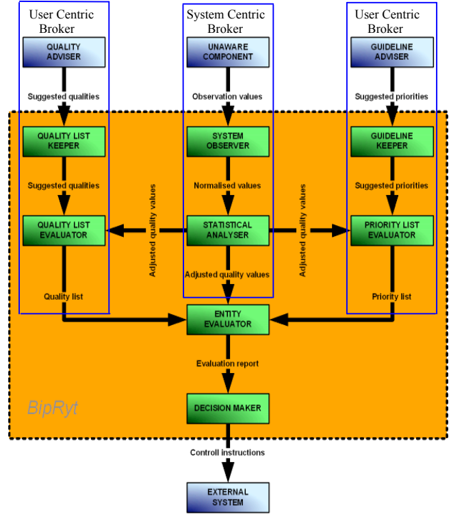
Fig. 6. Architectural Model of the BipRyt System
