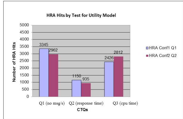
Fig. 15. Utility Model Adaptability to AHP Trend
