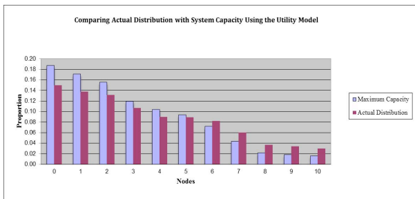
Fig. 20. The Utility Model Distribution vs. System Capacity
