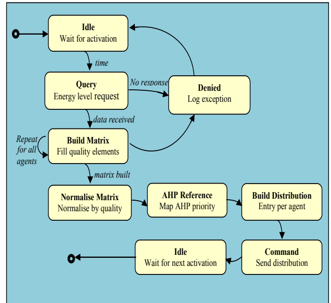
Fig. 8. Overview of decision-making processes
