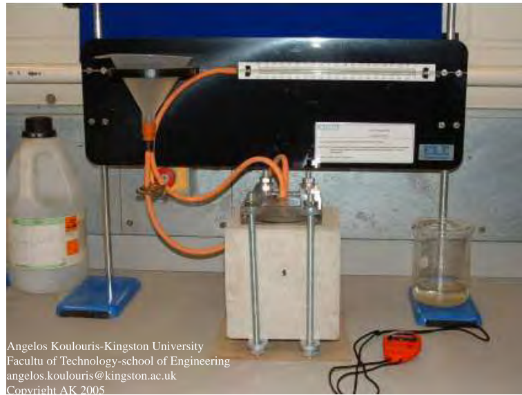
Figure 4.10: I.S.A.T. apparatus used.
