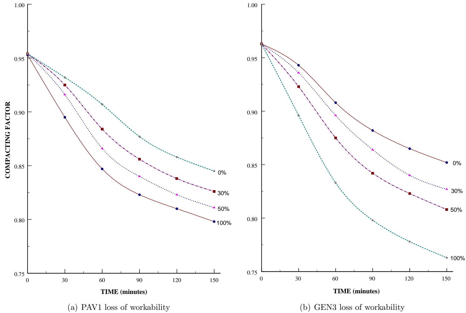
Figure 6.2: Effect of RCA content on the loss of workability over time for PAV1 and GEN3 concrete.
