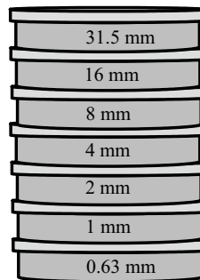
Figure 4.5: EN 933 size sieves assembled in column format
