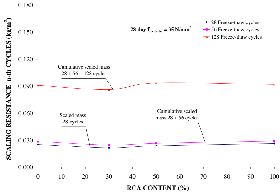
Figure 8.13: Effect of RCA content on the scale resistance of PAV2 concrete exposed to freeze-thaw cycling.
