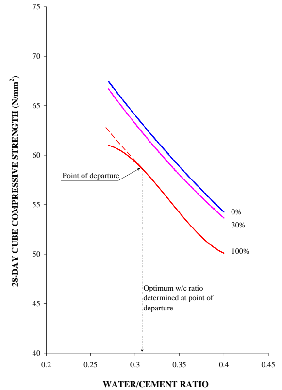
(c) 28-day compressive cube strength
