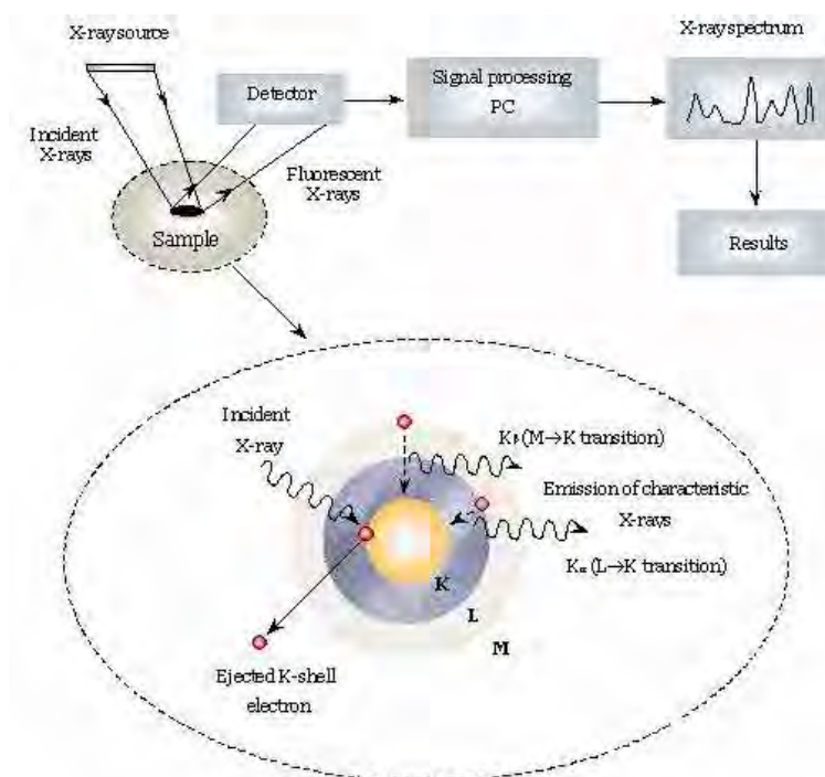
Figure 4.7: Principle of XRF analysis
