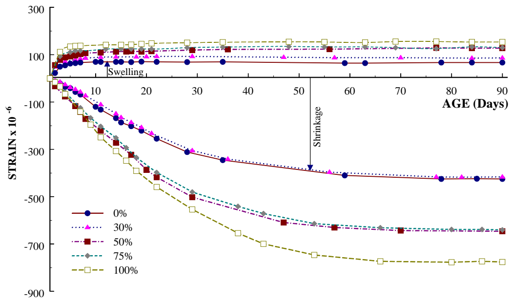
Figure 7.13: Effect of RCA content on deformation of PAV1 concrete.
