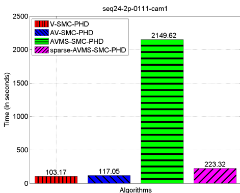
Fig. 10: Computational cost comparison between the V-SMC-PHD, AV-SMC-PHD, AVMS-SMC-PHD and sparse-AVMS-SMC-PHD filters.
