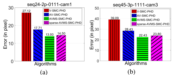
Fig. 12: Performance comparison of the V-SMC-PHD with the proposed algorithms AV-SMC-PHD, AVMS-SMC-PHD and sparse-AVMS-SMC-PHD with bar plots.
