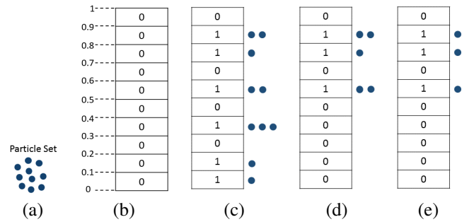
Fig. 3: A set of 10 particles is given in (a). Initial \mathbb{B} is illustrated in (b), and the distribution of the particles on \mathbb{B} according to Bhattacharyya coefficients is shown in (c). The updated \mathbb{B} after the estimation of the number of particles with KLD-Sampling is given in (d). Sparse particle selection is shown in (e).
