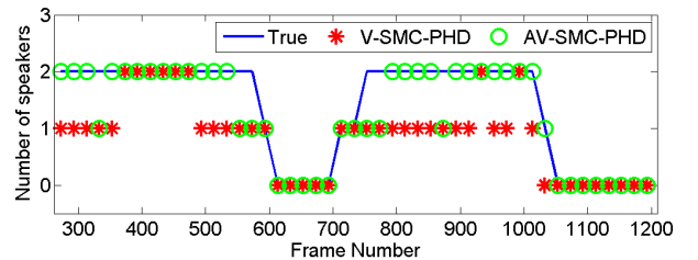
Fig. 6: Comparison of the V-SMC-PHD and the proposed AV-SMC-PHD filters in estimation of the number of speakers for Sequence 24 camera #1.
