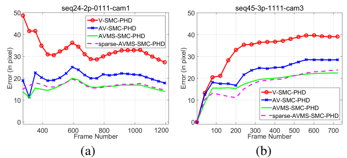
Fig. 11: Comparison of the V-SMC-PHD and the proposed algorithms AV-SMC-PHD, AVMS-SMC-PHD and sparse-AVMS-SMC-PHD using mean absolute OSPA-T error. The data points on the V-SMC-PHD curve were down sampled for better visualisation.
