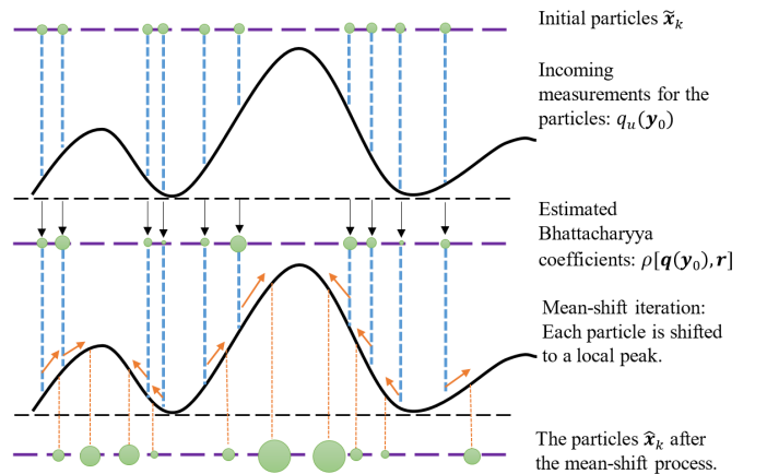
Fig. 2: The mean-shift process for the particles.
