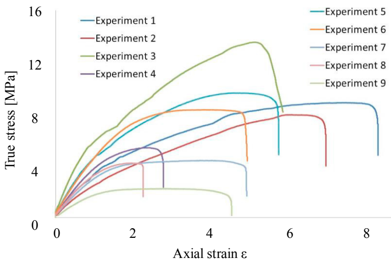
Fig. 3. Stress-Strain diagrams.
